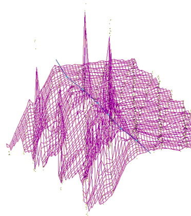
Figure 5: 3D modelled breakline determined on the basis of unclassified ALS data.
