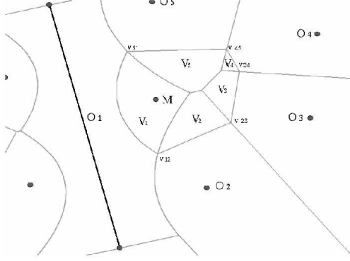
Figure 2: Natural neighbour interpolation
