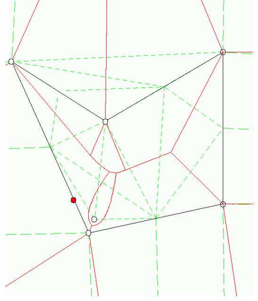
Figure 1: The Voronoi diagram of a set of points and line segments
