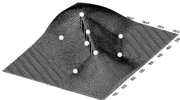
Figure 7: The surface obtained from the same data after using an Hermitian smoothing function, the data objects are marked by plain disks, the scale has been reduced in order to see the whole top surface
