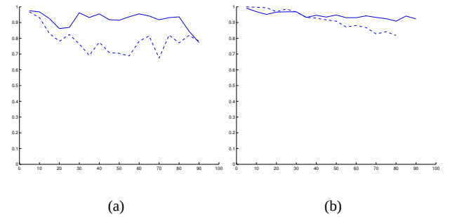
Figure 6: Illustration of the invariance against viewpoint changes: The rotation between the two cameras is increased in five degree steps from five to ninety degrees. The continuous line is the result for our approach, the dashed lines is for the centered support region. (a) shows the results for the data of the turntable sequence for real images. The variance results from occlusion effects, when new faces appear or other vanish. (b) illustrates the results for the synthetic turntable sequence.
