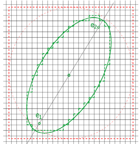
Figure 3. Ellipse (green solid line) with check area (red dashed), finally selected pixels (green dashed). Expected area 221 (=11x11) and finally selected pixel 218, representing differentiation less than 1.5%.
