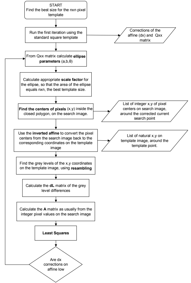
Figure 1. Flow chart of the implemented method.
