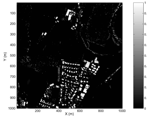
Figure 3. The joint membership function ( MF_{OA} ) for extracting buildings based on both measure ( MF_{Seg} and MF_{NDVI} ).
