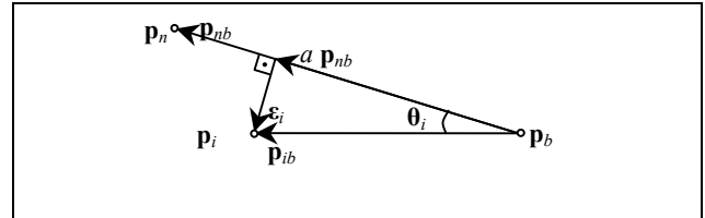
Figure 2. Geometric interpretation of the spectral response model for pixels crossed by unpaved roads.
