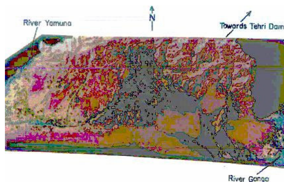
Fig. 2 Land Cover Themes – IRS LISS-II November 1993
