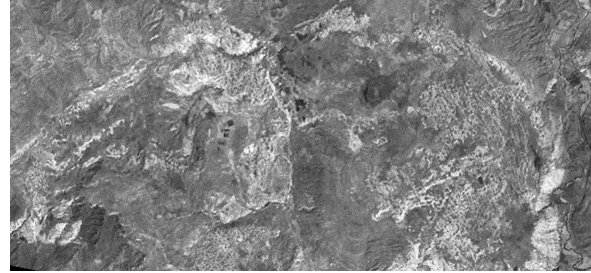
Figure 2: Décollement gypsum levels on band 5, Landsat ETM+ image are highlighted in white.
