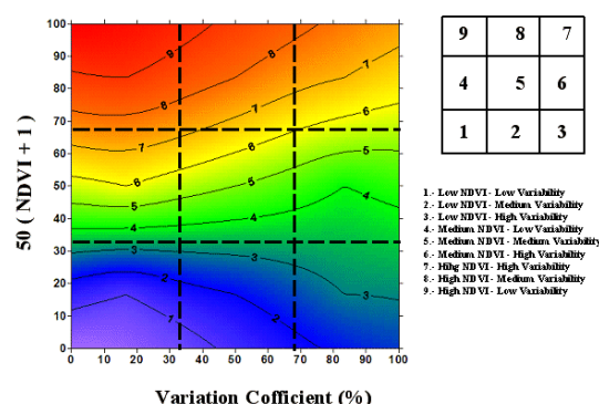
Figure 2.- Proposed relation for the study area classification. It is based on the variability among the time series, and its absolute maximum values. This corresponds to the used classification matrix.
