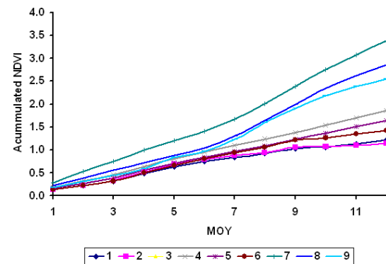
Figure 6.- Accumulated NDVI month by month.
