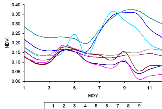
Figure 5.- Mean monthly evolution of the NDVI for each SHI class
