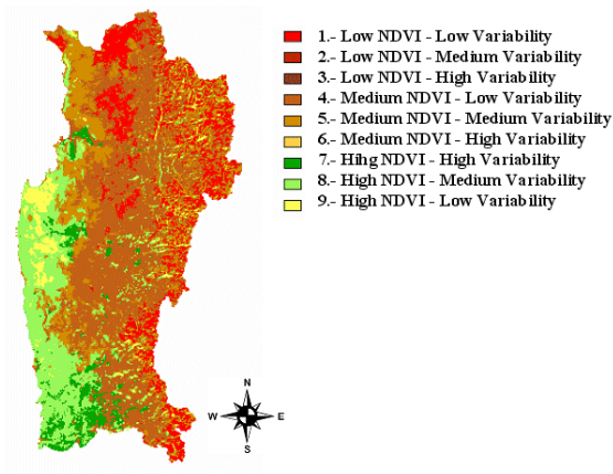
Figure 3.- Spatial homogeneity index (SHI) which relates the mean maximum values and the variation coefficient. As a general norm, increased NDVI means better ecosystem quality, and increased variability means an increase in the ecosystem instability.
