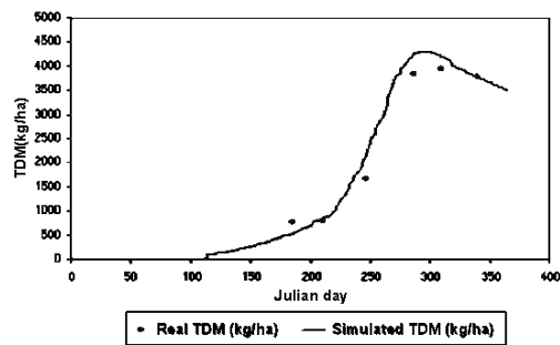
Figure 7.- Variation of the total dry matter (DM) accumulation according to the Julian day. Simulated values (—) and the real values (•) measured in field experiment. Hidango, season 1992.
