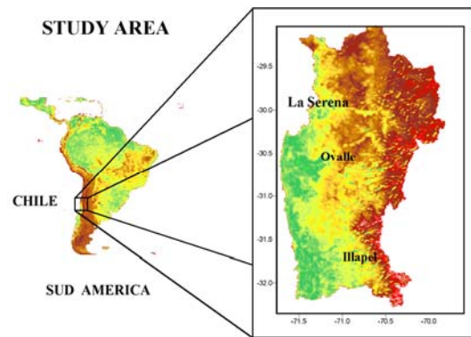
Figure 1.- Study area: Limari province, which is located in the IVth region of Chile. This zone corresponds to a transition between the arid climate and the Mediterranean one known as a semi-arid zone.
