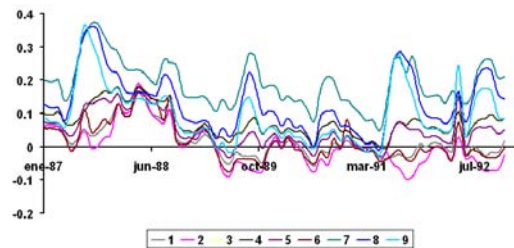
Figure 4.- Monthly evolution of the NDVI for each class of the SHI in the time series of NOAA-AVHRR images.
