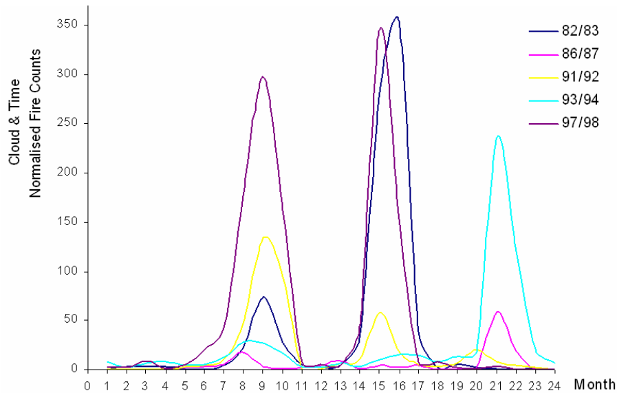
Figure 2 Active Fire Counts from AVHRR GAC data of Borneo for the 24 month period surrounding five individual ENSO episodes. The strong seasonality of fire activity in Borneo is clearly depicted in all five ENSO events, with the majority occurring in August-October of Year 0 or Year 1, and February-March-April of Year 1. The strongest and most prolonged El Niño events (i.e. 1982-83/1997-98 and 1991-94 respectively) were accompanied by the most extreme fire occurrence.
