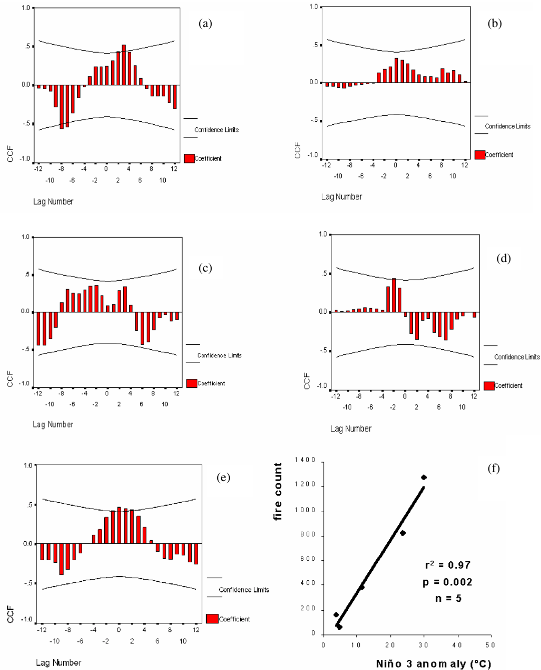
Figure 3 (a-e) The correlation coefficient (CCF) of Niño 3 anomaly-fire count at various lag times (i.e. negative lag number). Positive lag numbers (lead time) were ignored since current and past fire events cannot be explained and attributed to future ENSO variations. The higher the coefficient the stronger the ENSO-fire correlation; horizontal black line depicts the 0.5 confidence limits; (a) 1982-83, (b) 1986-87, (c) 1991-92, (d) 1993-94, and (e) 1997-98. (f) The 16-month sum of Niño 3 anomaly, from January of Year 0 to April of Year 1, versus the 16-month cumulative all-Borneo fire counts over the same time period for the five El Niño events studied.
