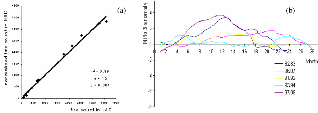
Figure 1 (a) Regression analysis between LAC and adjusted GAC fire counts during El Niño period. (b) Temporal evolution of Niño 3 anomaly during the five El Niño events studied herein. It is clearly indicated the two strongest El Niño events of 1982-83 and 1997-98, these having the highest absolute anomaly values. These data were obtained from the Climate Prediction Centre of the NOAA National weather Service in USA.
