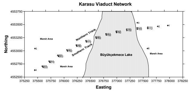
Figure 1: The configuration of geodetic network.
