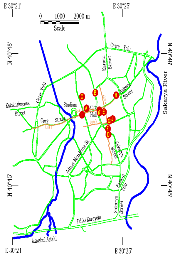
Figure 5. Measurement sites in Sakarya
