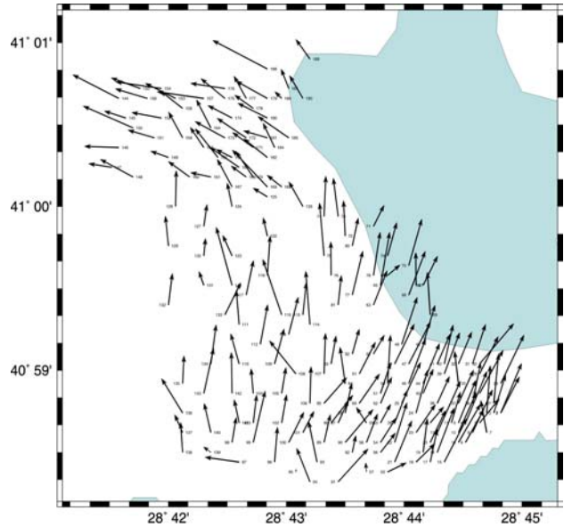
Figure 7. Displacement vectors for horizontal coordinates between the years 1999 and 1987
