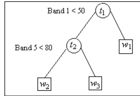
Figure 1. Example of decision tree using synthetic data
