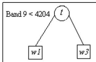
Figure 4. Decision tree to separate Woods ( w_1 ) from Corn ( w_3 )
