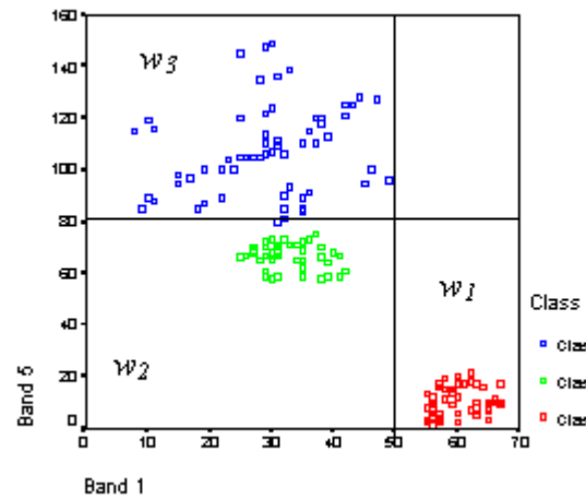
Figure 2. Subdivisions of the feature space determined by the decision tree (synthetic data)
