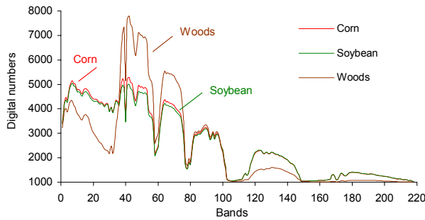
Figure 3. Mean spectral behaviour of the three classes denoted by woods, soybean and corn
