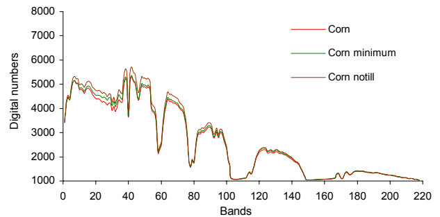
Figure 5. Mean spectral behaviour of the three classes denoted by corn, corn minimum and corn no till
