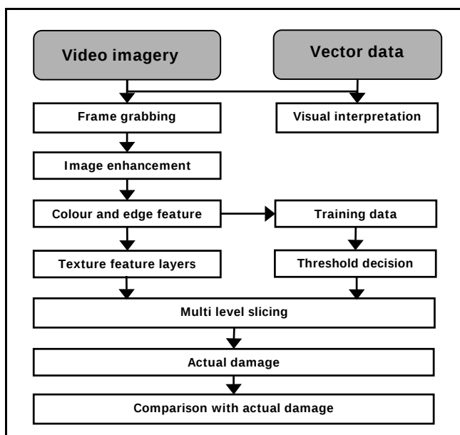
Figure 3. Damage assessment using video imagery
