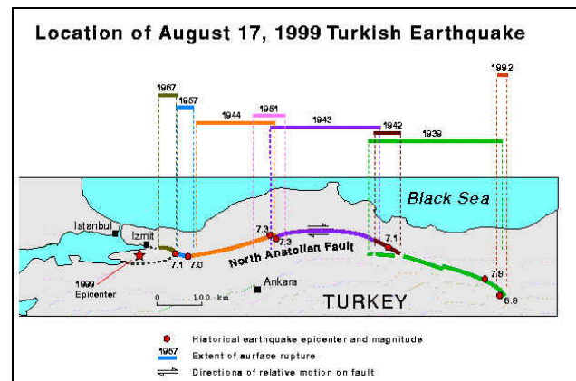
Figure 1. North Anatolian Fault Zone and case study area ( http://geohazards.cr.usgs.gov accessed on 14 November 2003)
