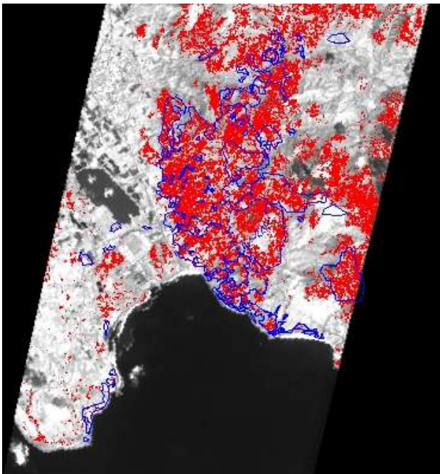
Figure 5. Preliminary result (red) from spectral analysis and known ground truth data (blue).
