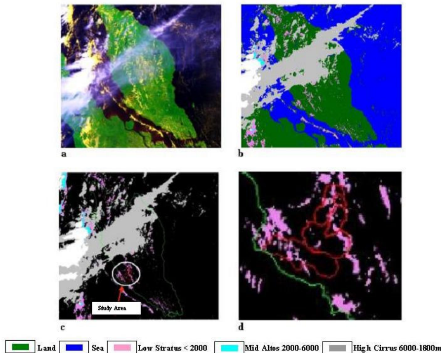
Fig 4 Cloud Type Identification and Classification
