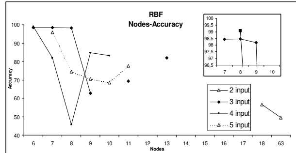
Figure 7. RBF overall accuracy according to nodes
