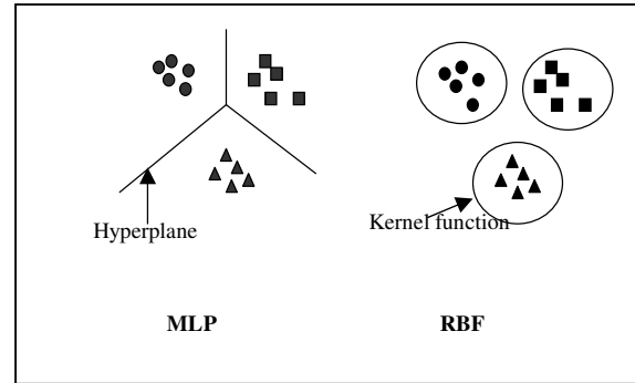
Figure 3. MLP and RBF classification approach
