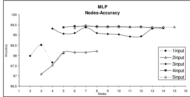
Figure 6. MLP overall accuracy according to nodes
