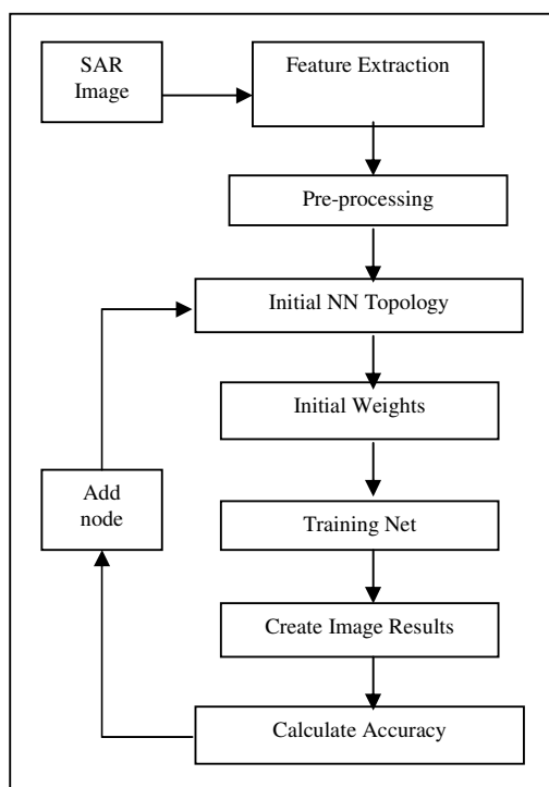
Figure 4. Methodology used
