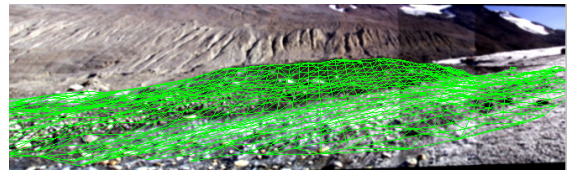
Figure 4. The terrestrial DEM of Hintereisferner test field in September 2002.
