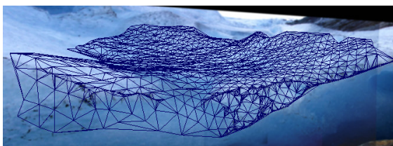
Figure 2. DEM of Engabreen test area in 2001
