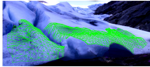
Figure 3. DEM of Engabreen test area in 2002
