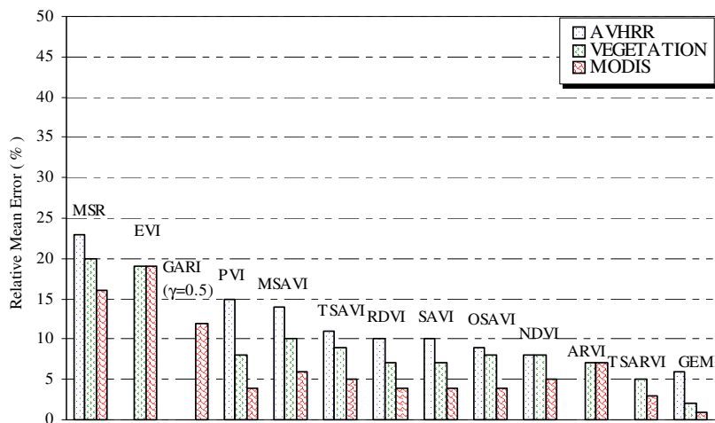
Figure 1: Sensitivity of different vegetation indices to ozone concentration (0,959 g/cm 3 ) considering a dense forest cover (100 %).
