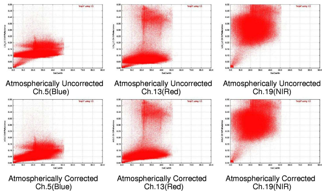
Figure.4: Satellite Zenith Angle vs. Atmospherically Uncorrected/Corrected Reflectance on GLI 1km 16-day VGI(NDVI,EVI) composite
