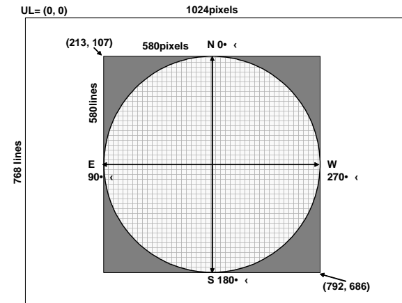
Figure 2. Hemispherical area and image coordinates
