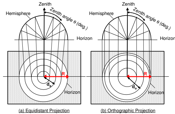
Figure 1. Projections of fisheye lens Left: Equidistant Projection, \theta/90 = d_c/R Right: Orthographic Projection, \sin \theta = d_o/R
