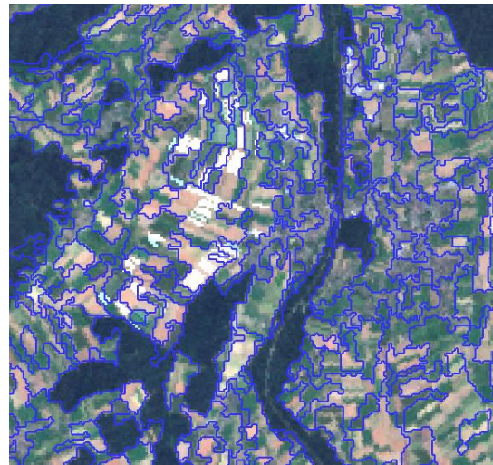
Segmentation level 3
