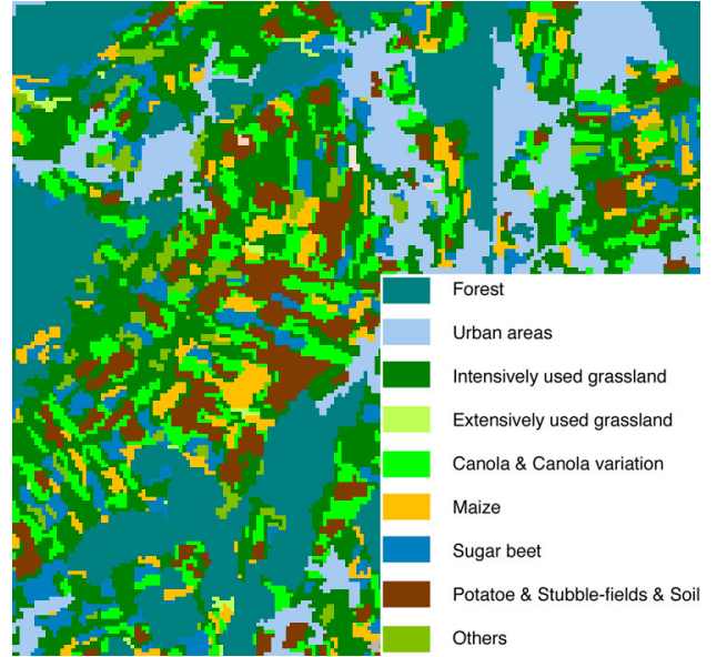
Figure 4. Land use classification result based on object-oriented classification method with eCognition.
