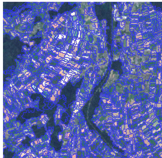
Segmentation level 2
