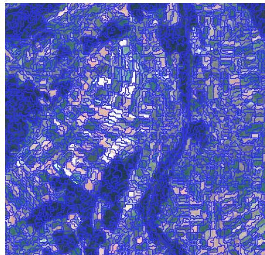
Segmentation level 1
