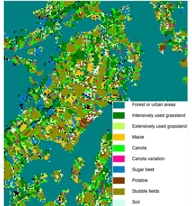
Figure 3. Land use classification result based on a Spectral Angle Mapper (SAM) approach.
