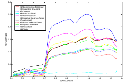
Figure 6. The mean spectra of 11 different classes
