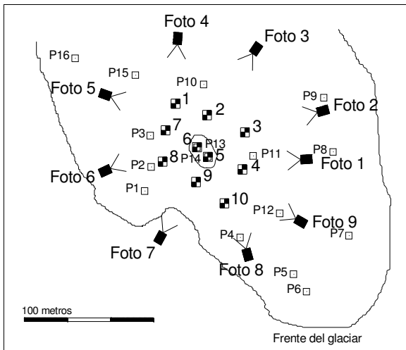
Figure 4. Scheme of the rods, control points or artificial signs of the photographs takings.
