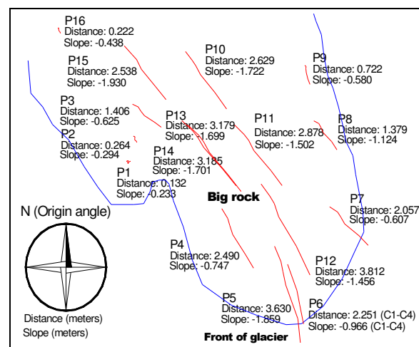
Figure 2. Dynamic of Argualas glacier (1991-2000).
