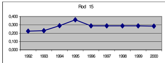
Figure 3. Glacier dynamic of rod number 15.
