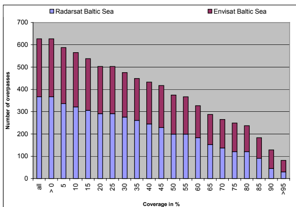
Figure 4. Yearly RADARSAT and ENVISAT coverage of the German EEZ in the North Sea
