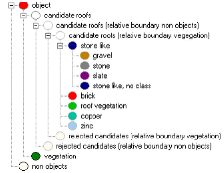
Figure 10: Class hierarchy
