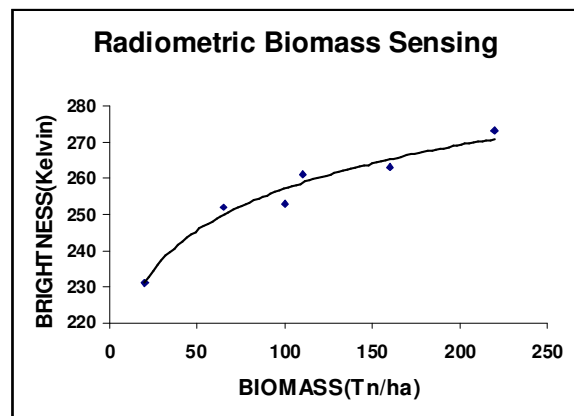
Figure 5. Brightness temperature vs. biomass
