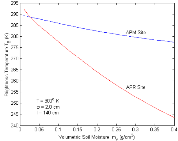
Figure 9. Model variation of brightness temperature with soil moisture for the APR and APM sites.
