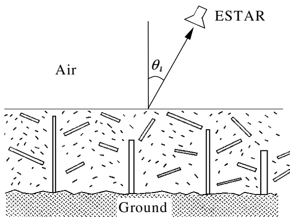
Figure 6. The forest model
