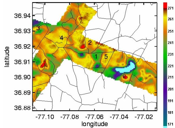
Figure 4. ESTAR brightness temperature maps for flights on November, 15, 1999
