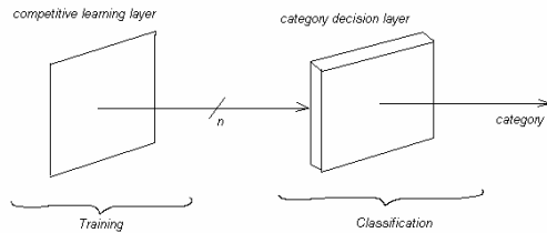
Figure 1. A modified competitive learning neural networks with the extension of a category decision layer.
