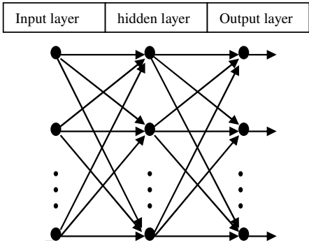
Figure 2. A backpropagation feed-forward multilayer neural networks.
