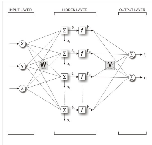
Figure 2 - MLP NN mathematical model with 2 computational layer ( hidden e output ) designed for the ortho-correction problem.
