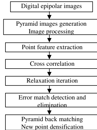
Figure 1: Workflow of matching
