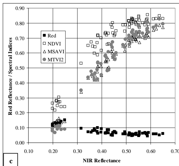
Figure 1. Sensitivity of red reflectance, NDVI, MSAVI2 and MTVI2 to changes in the NIR reflectance of crop canopies (Corn (a), Beans (b), and Peas (c)). Data are from the campaign of 2003.
