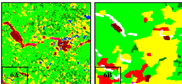
Figure 6: The pixel-based classification in a masked area (6A) and the object-oriented classification in the same area (6B). See salt-peppery image at the pixel-based method.
