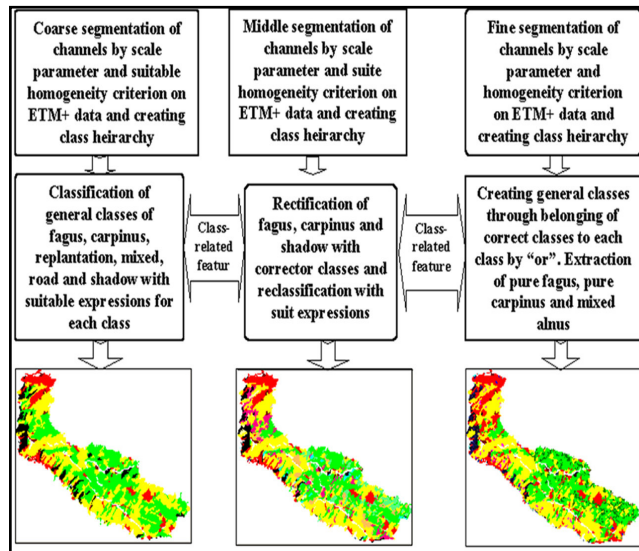
Figure 4: Flowchart of hierarchical forest types classification by membership function method on ETM+ bands and their results in each level
