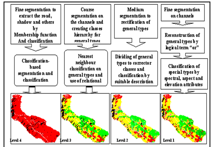
Figure 5: Flowchart of hierarchical forest types classification by integration nearest Neighbour & Membership function and results in each level.
