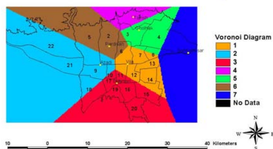
Figure 6. Voronoi Diagram of Tehran's air pollution monitoring stations
