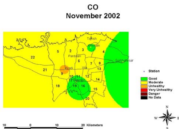
Figure 3. Spatial dispersion of co in November in 2002
