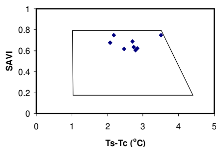
Figure 6 Temperature difference – SAVI trapezoid of alfalfa adjusted vegetation index.
