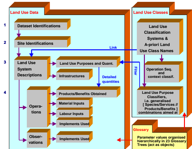
Figure 4. The underlying database files on Land Use (4 main levels); Squares represent one database file each, links from the (23) Glossary files to the ; Land Use Data and Land Use Classes data files are not shown in detail.
