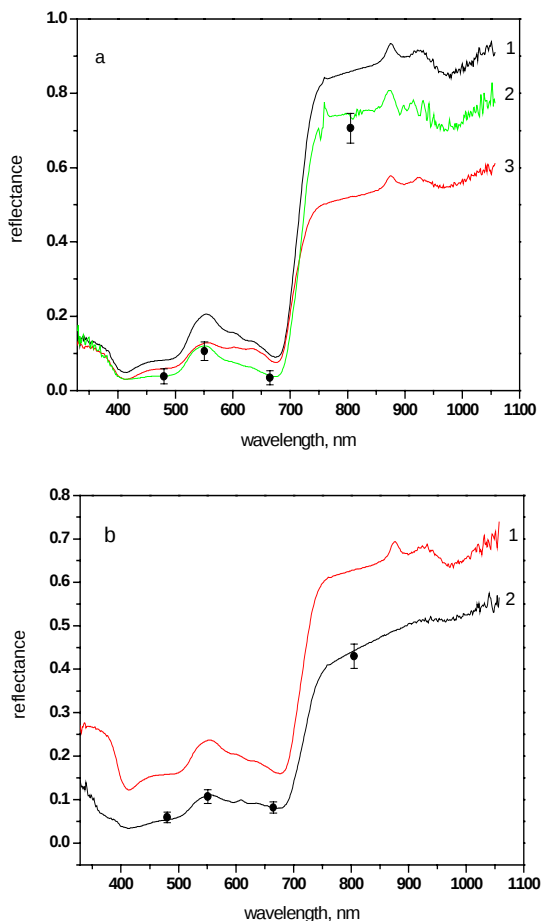
Figure 1. Solar radiation reflectance spectra from different objects, gained by ground spectroscopy method (solid curve) and satellite data IKONOS (dots):
