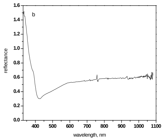
Figure 2. Solar radiation reflectance spectra from contiguous plants from the sites of wild hemp vegetation of Shu valley (solid curve- ground spectroscopy, dots- satellite data IKONOS)
