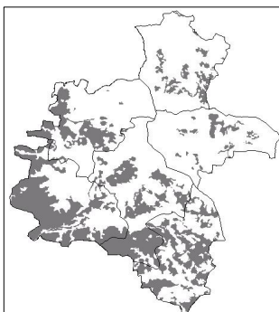
Figure 4B: Conservation
