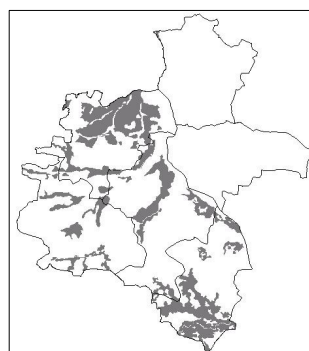
Figure 4C: Crop-Selection
