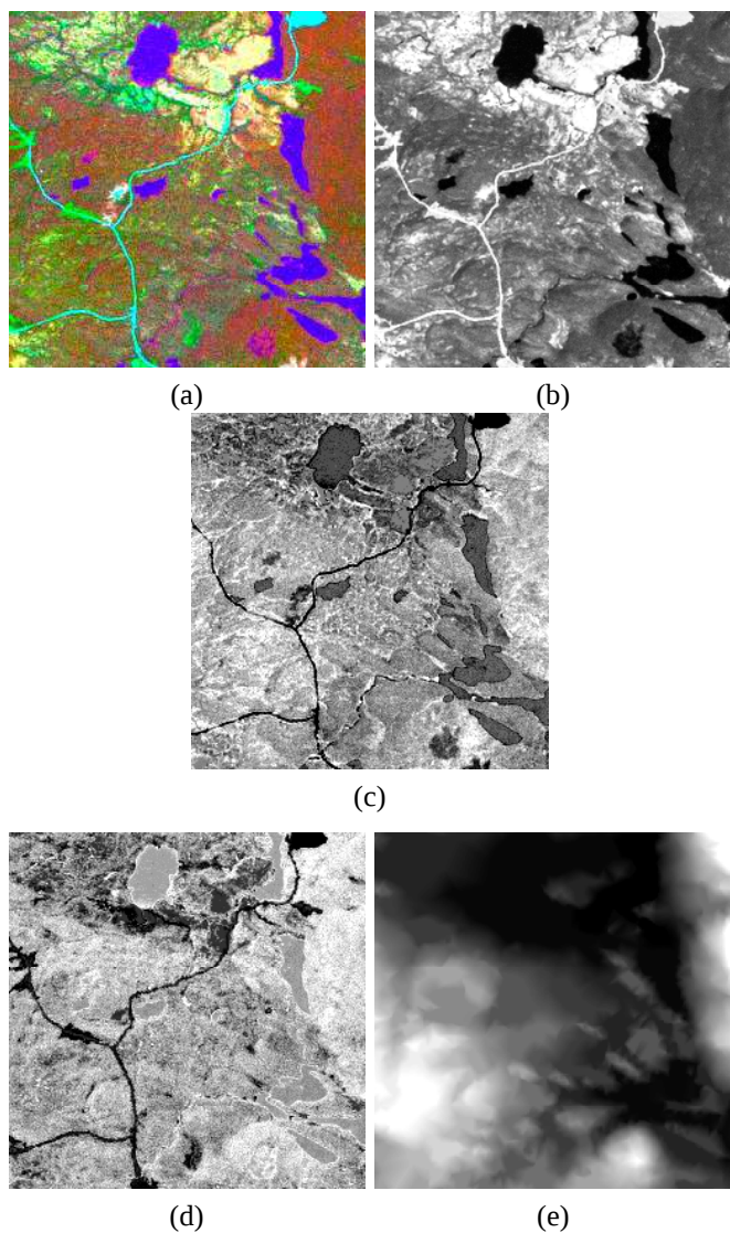
Fig. 1. (a) image composed of 3 principal components from LANDSAT TM multispectral images, (b) to (d) Brightness, Greenness, and Wetness Tasseled Cap indices respectively, (e) Altitude information
