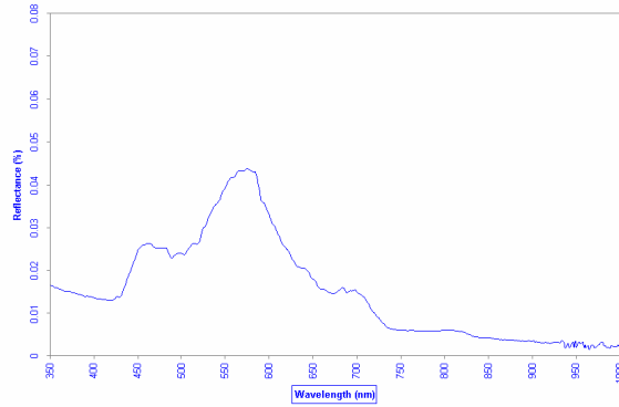
Figure 10. High resolution spectra of Kentucky Lake (the scale is between 0 and 1 (100%) for the reflectance axis)
