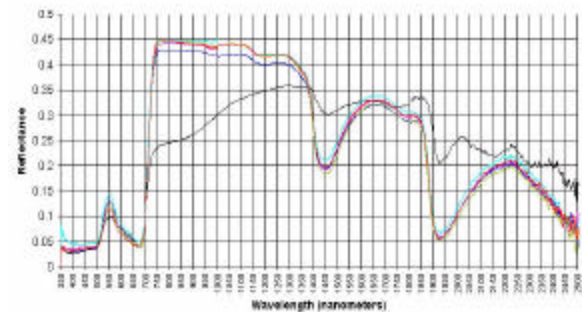
Figure 9. Spectra of black willow; healthy and under stress (the scale is between 0 and 1 (100%) for the reflectance axis)
