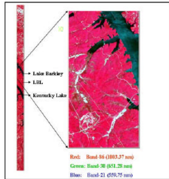
Figure 2. The Hyperion dataset, April 29, 2001
