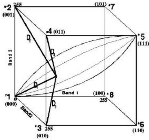
Figure 6. nPDF Cube Model
