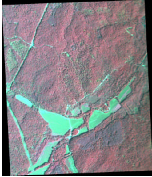
Red: Band 110 (850nm),_Green: Band 60 (650nm), Blue: Band 35 (550nm)
