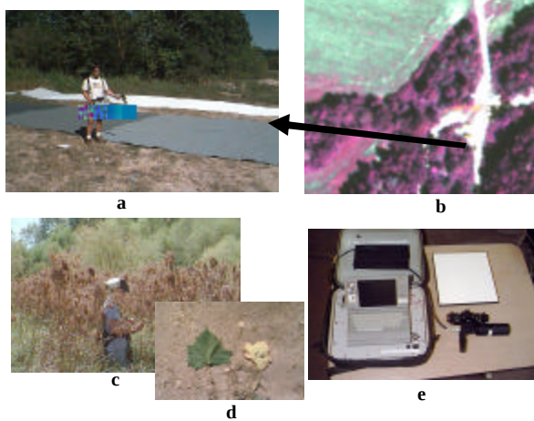
Figure 4. a) Gray-scale placards, b) RDACS imafe showing the location of the placards, c) GPS measurement, d) sycamore leaves; healthy and under stress, and e) Full range (350-2500nm) field spectroradiometer used in this study
