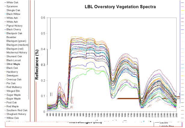
Figure 5. Spectra of the vegetation species in LBL
