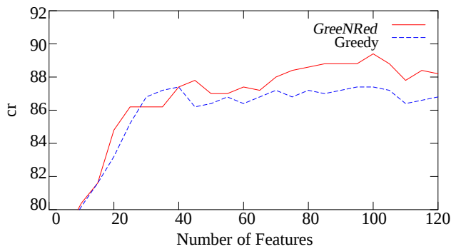
Figure 3: GreenNRed -greedy comparison with the 3-NN algorithm
