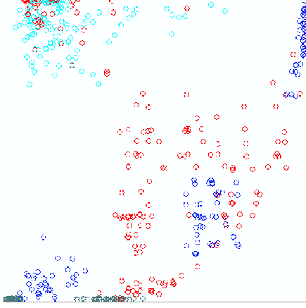
Figure 2: Projection of samples in the RED-NIR plane.
