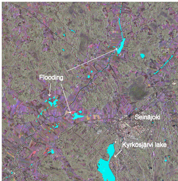
Figure 1. Snowmelt caused a minor flooding in April 2001. Original data © distributed by Radarsat International/TSS/Novosat Ltd. Processed by FGI.
