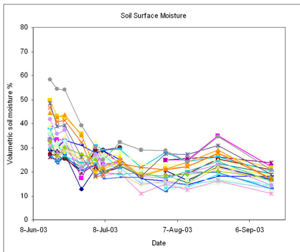
Figure 4. Volumetric soil surface moisture for test parcels in summer 2003.
