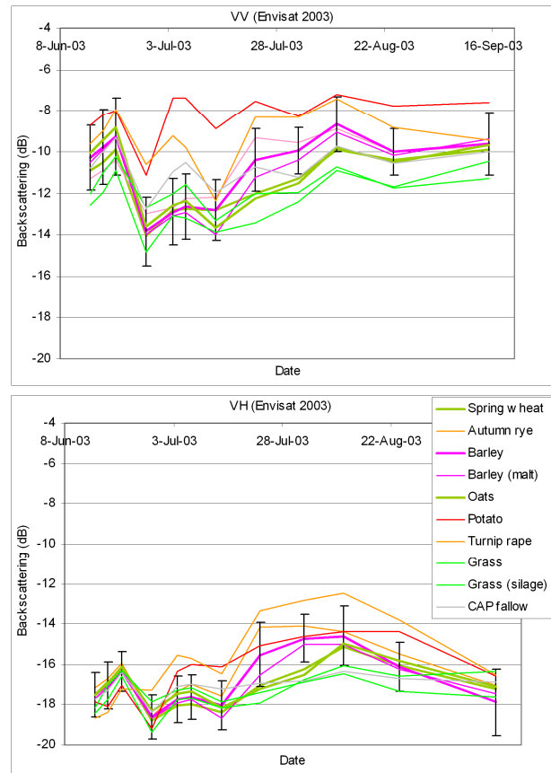
Figure 3. Time series of SAR backscattering in VV and VH polarizations for major crop species in 2003 in Finland.
