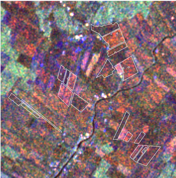
Figure 2. A multitemporal dual-polarization Envisat SAR image from the Seinäjoki test area in summer 2003. Original data © European Space Agency. Processed by FGI.
