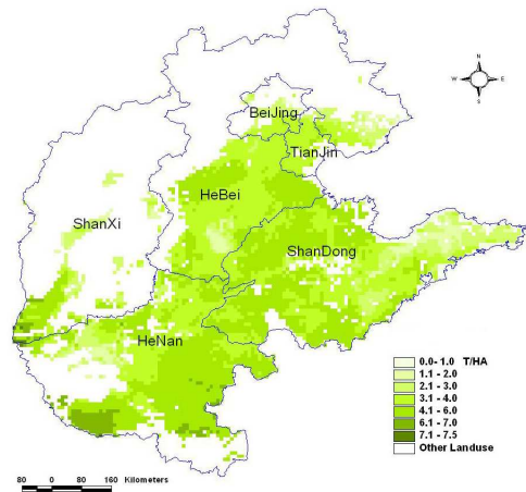
Figure 3. The simulated yield per hectare of summer corn by spatial EPIC model in North China
