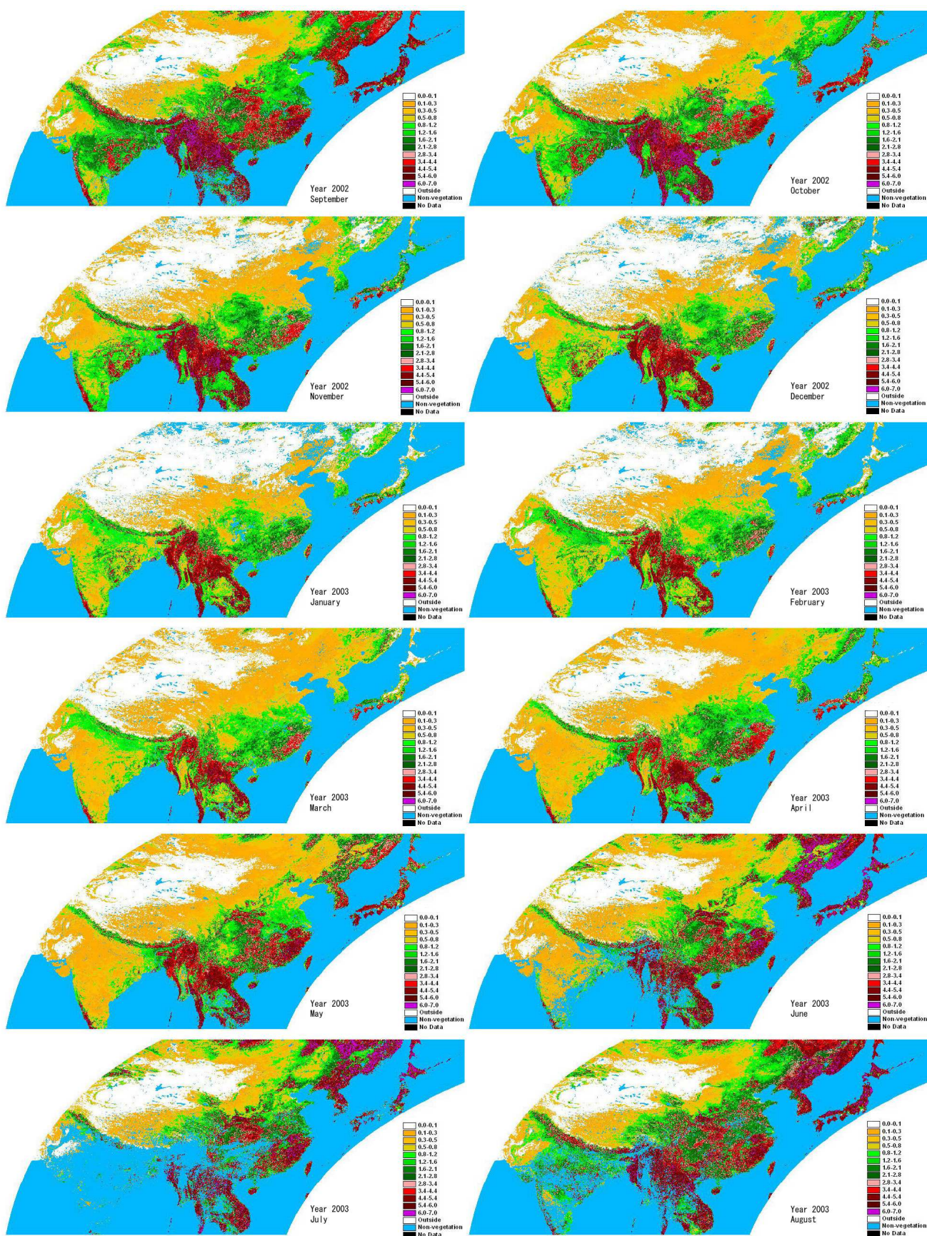
Figure 4. Colour-coded images of monthly MODIS LAI product for East Asia from year 2002 (September) to year 2003 (August)
