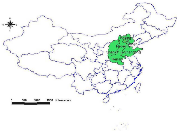
Figure 1. The study region of North China covers a 6.9 \times 10^5 km 2 area (110°E-123°E longitude and 30°N-43°N latitude)
