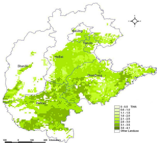
Figure 2. The simulated yield per hectare of winter wheat by spatial EPIC model in North China
