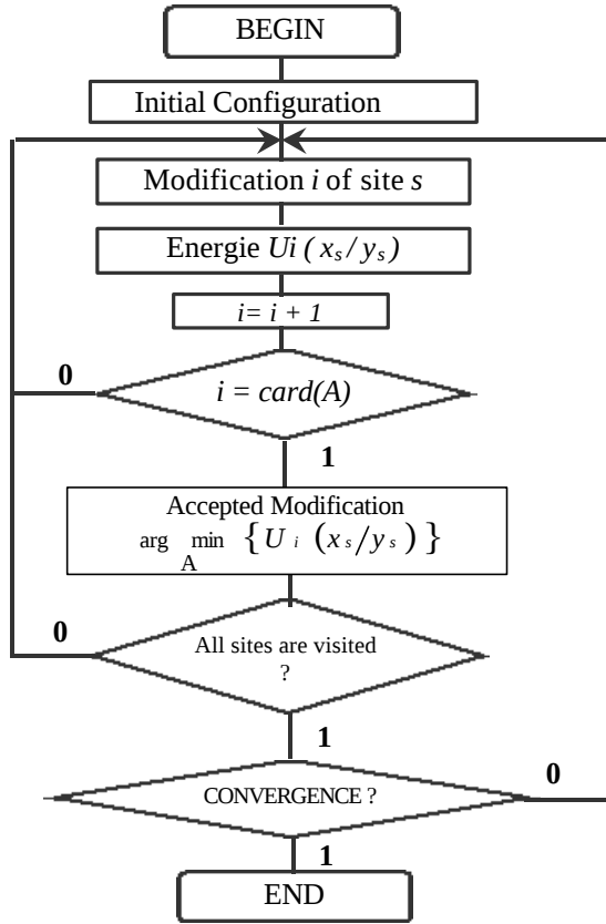
Figure 2. ICM flow chart
