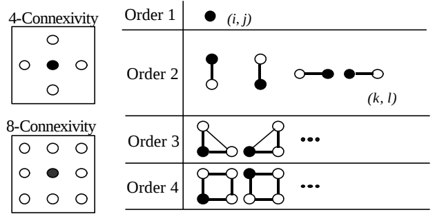
Figure 1. Neighbourhood and cliques
