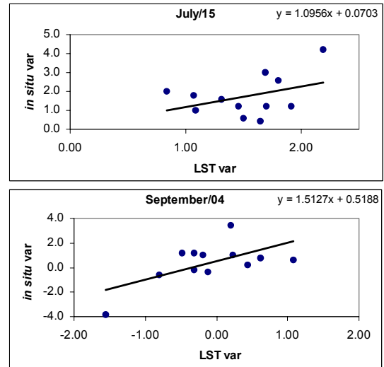
Figure 1. Scatterplot of LST and T_{air} ( in situ ) variation between two overpasses during night-time.
