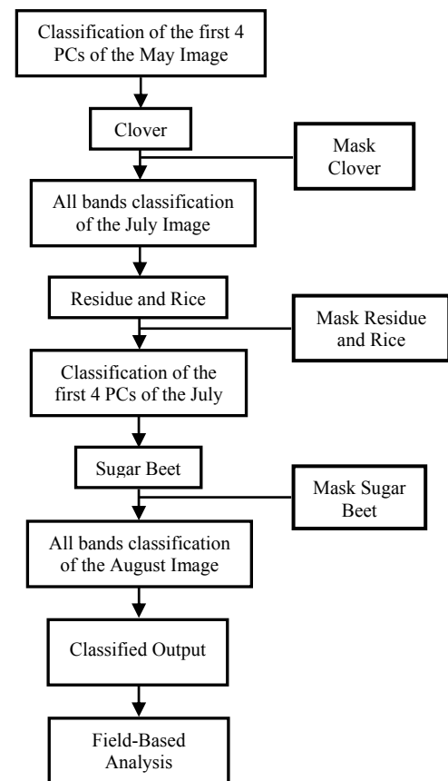
Figure 2. The sequential masking classification procedure.
