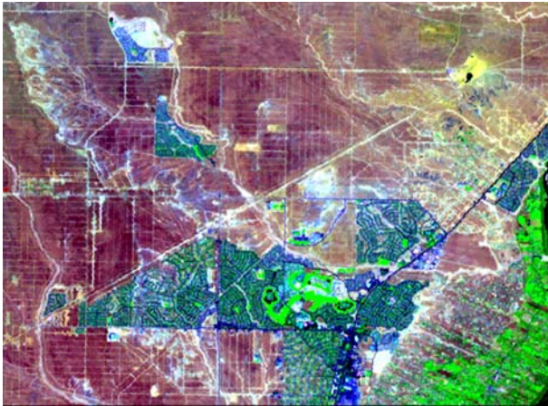
Figure 1. ETM+ image with 3 bands TM1, TM4, TM6 displayed in blue, green, and red, respectively
