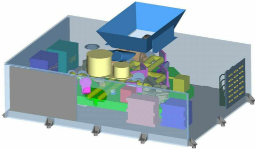
Figure 2. Instrument configuration.
