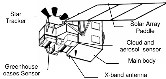
Figure 9. GOSAT on orbit.
