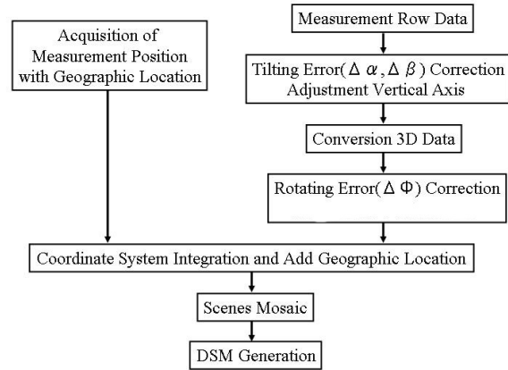
Figure 7. Data Processing Procedure
