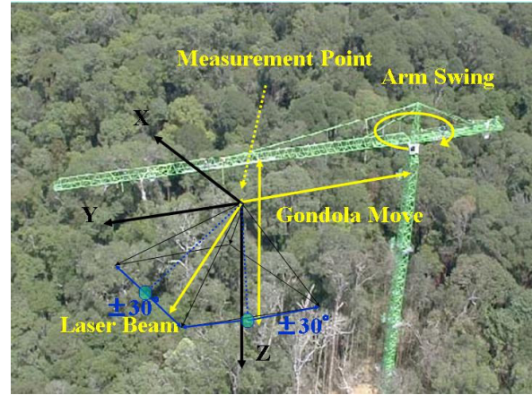
Figure 3. Concept of 3D Measurement using Canopy Crane
