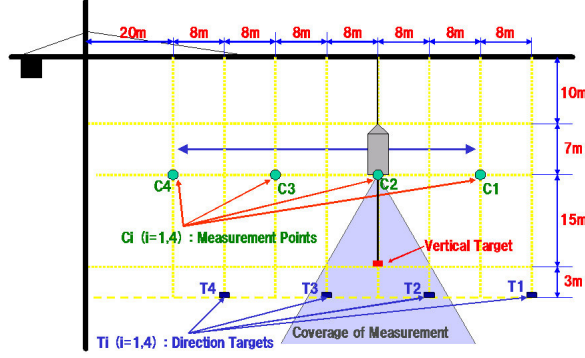
Figure 5. Measurement Coverage and Deployment of Correction Targets
