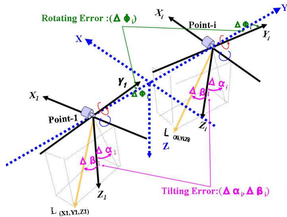
Figure 4. Measurement Geometry
