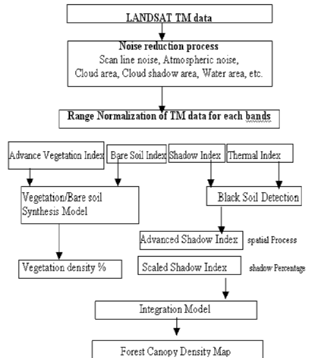
Figure 4. Flow chart of FCD Mapping Model
