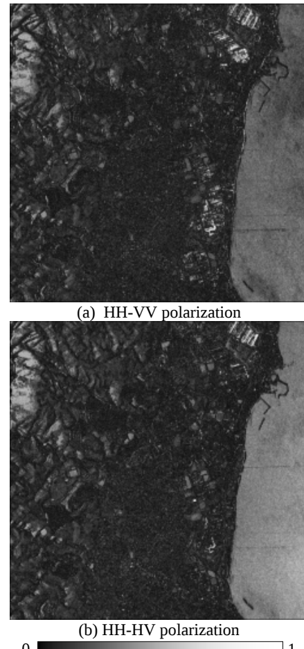
Figure 4. Example of Rajsiki distance image for Pi-SAR Hitachi site X-band data (2002)
