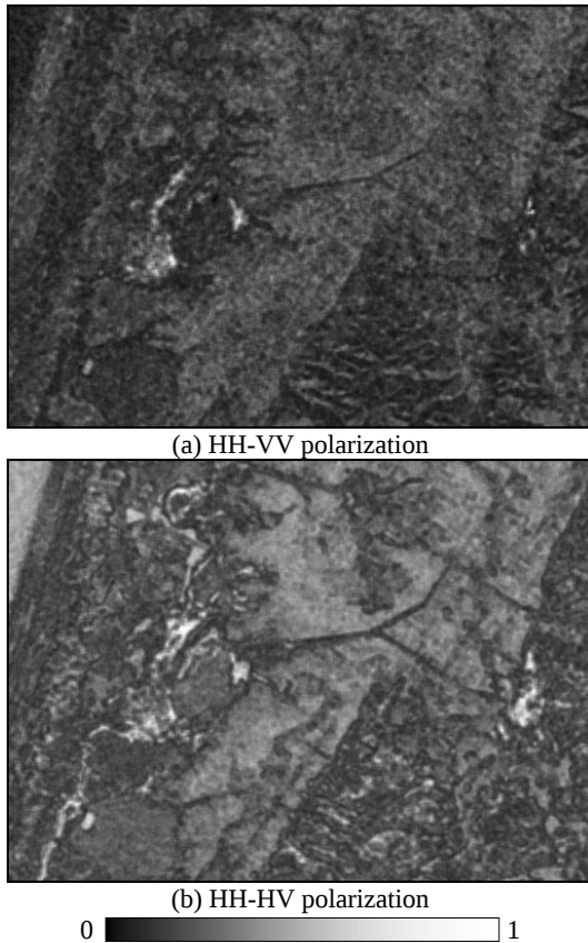
Figure 2. Example of Rajsiki distance image for SIR-C Sarobetsu site C-band data (1994)
