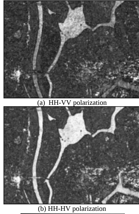
Figure 3. Example of Rajsiki distance image for SIR-C Kashima site C-band data (1994)
